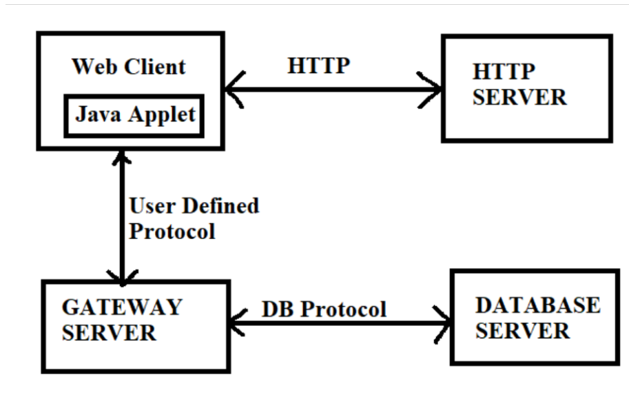
Figure: Architecture of Java Applet
