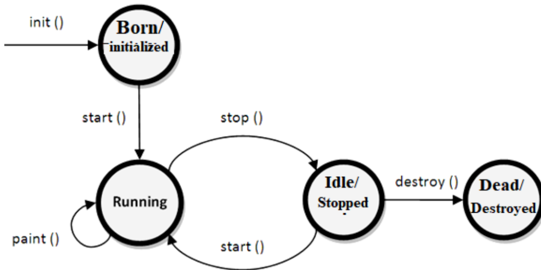
Figure: Life Cycle of an Applet.
